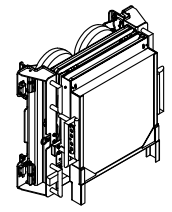
ISOMETRIC (STOWED VERT.)
