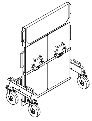
ISOMETRIC
